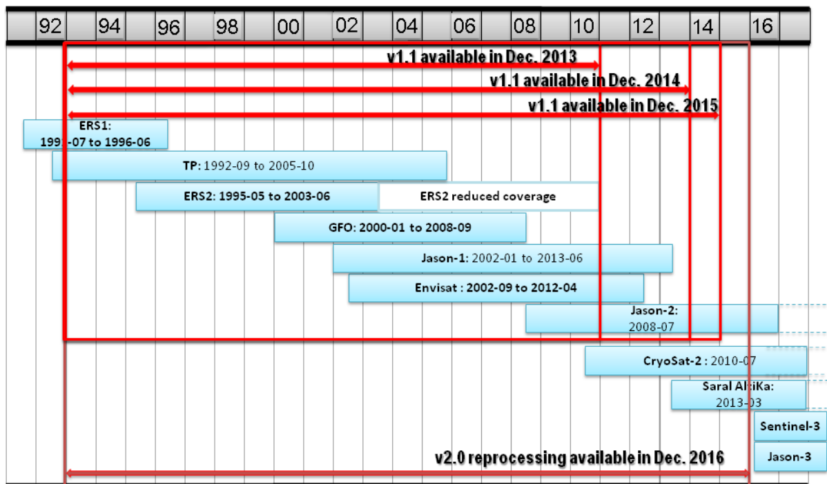
Figure 1: Level 2 GDR altimeter data, used as input data to generate the FCDR and ECV products, are included in the red squares according to the version of the product.
