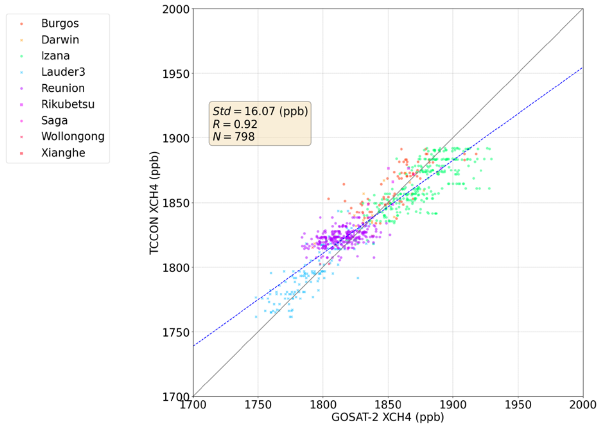
Figure 4.2 Same as Figure 4.1 but for soundings taken in glint mode.
