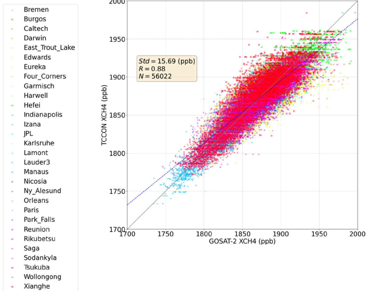
Figure 2: GOSAT-2 XCH 4 for soundings over land plotted against TCCON, for the RemoTeC Proxy product. Data are compared only if they are fully colocated in space and time. The standard deviation of the population, Pearson's correlation coefficient and number of retrievals are given in the inset. The legend plots the different TCCON stations where markers are as follows. Stations that are along the coast and also sensitive to glint mode (ocean) measurements are indicated as circles. Those that have high latitudes in the northern and southern hemispheres are upward triangles and crosses, respectively. Stations in Asia, North America and Europe are indicated by squares, pluses and downward triangles respectively.
