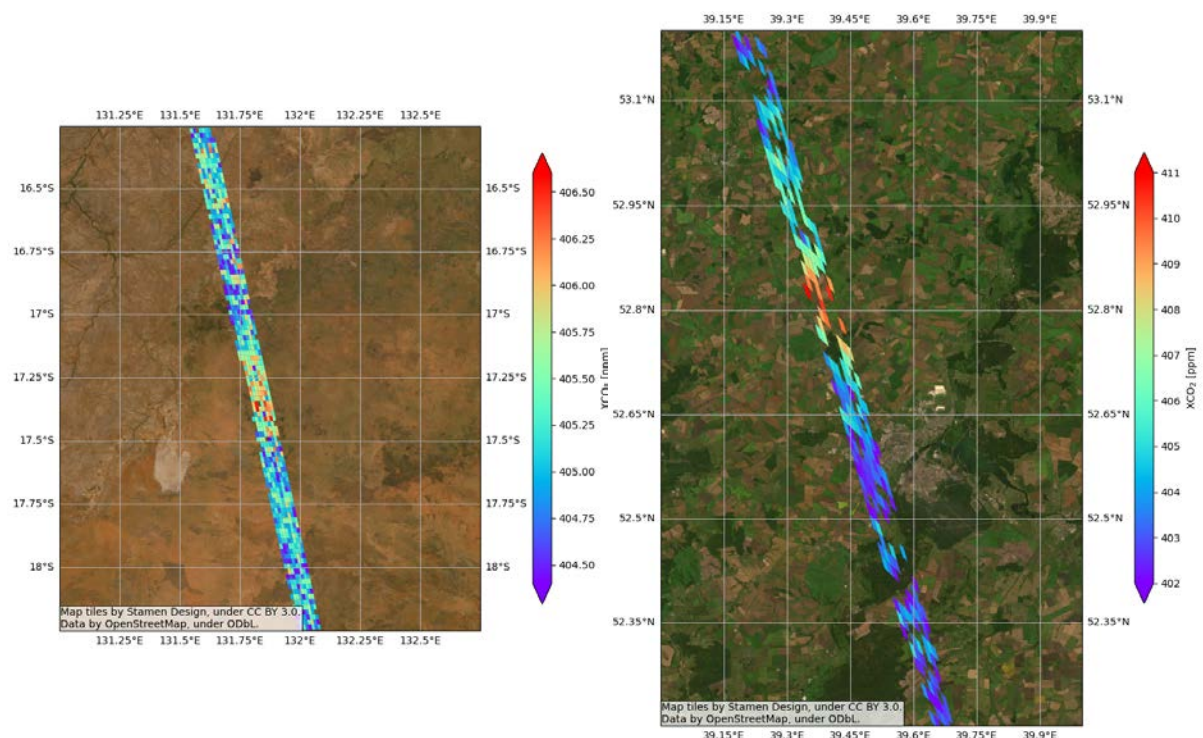
Figure 6.1: Left) Local XCO 2 enhancement due to emissions of Australian wildfires (May 5, 2018, 05:00 UTC). Right) Local XCO 2 enhancement due to the emissions of the TEC-2 Lipetsk power plant in Russia (August 25, 2018, 10:15 UTC).
