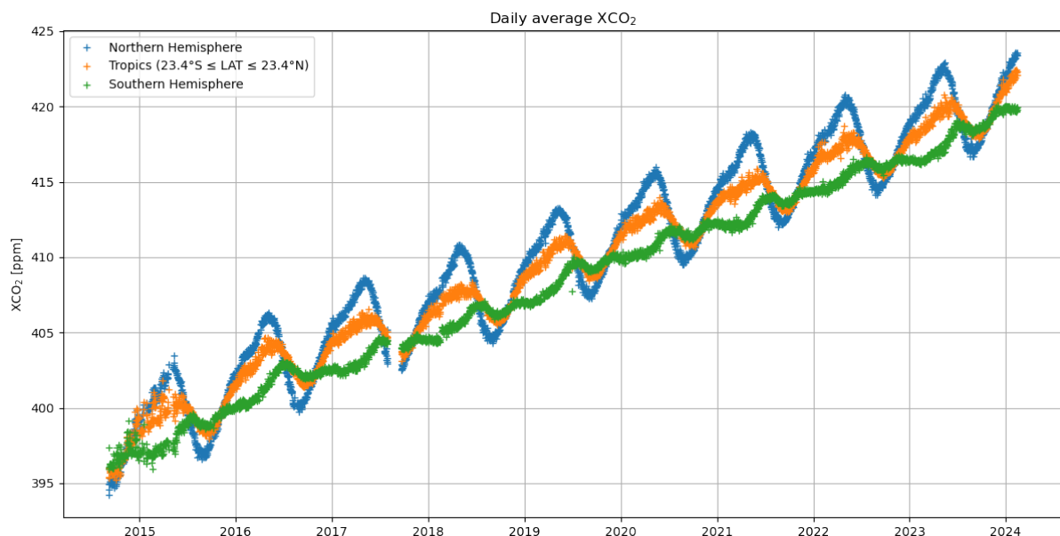
Figure 6.3: FOCAL XCO 2 daily averages of the northern hemisphere (latitude \geq 0^{\circ}\text{N} ), southern hemisphere (latitude < 0^{\circ}\text{N} ), and the tropics ( -23.4^{\circ}\text{N} \leq \text{latitude} \leq 23.4^{\circ}\text{N} ).
