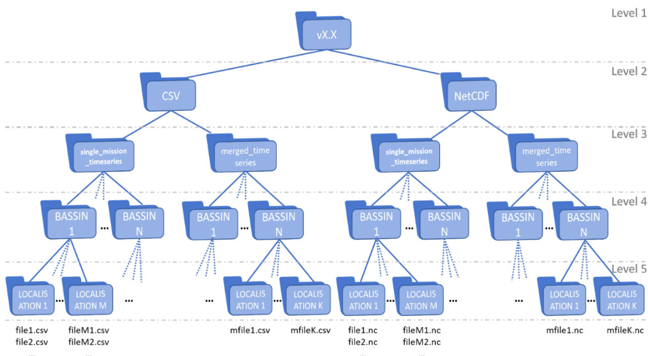
Figure 5. WSE CRDP directory structure
