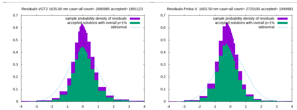
Figure 3: In purple: Residuals per sensor and band, contributing to the cost function vector after retrieval for the central-European tile X18Y02 (in PROBA-V nomenclature) for 2014-05-16. Left column: VGT2, right column PROBA-V; bands as indicated in sub-captions. In green: subset of inversions accepted by a chi-square test. Light blue line: density of the Gaussian distribution which would be expected if all assumptions were ideally fulfilled.
