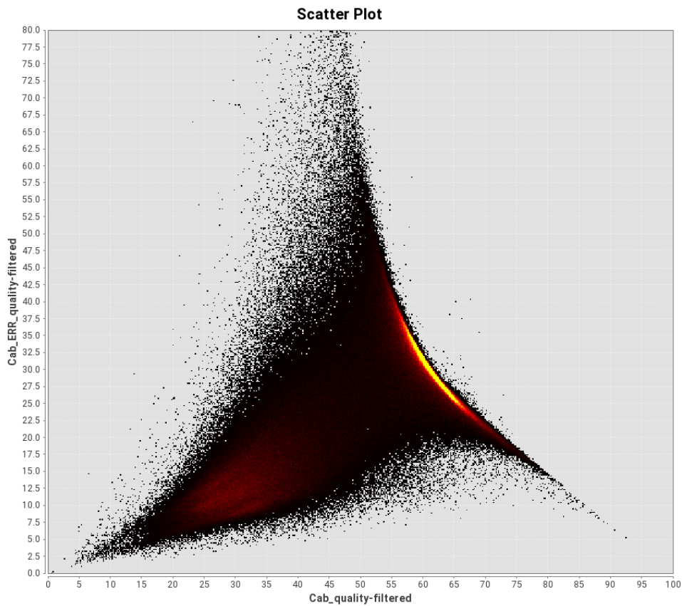
Figure 6: Scatter plot of OptiSAIL Cab uncertainty over the estimated quality-filtered Cab value from 2014-05-16 for the central-European tile X18Y02 (in PROBA-V nomenclature, units on both axes are \text{ug.m}^{-2} ).
