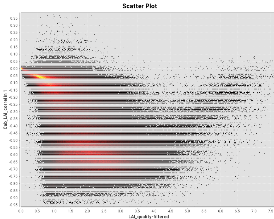
Figure 7: Scatter plot of Cab-LAI uncertainty correlation over the estimated quality-filtered LAI value from 2014-05-16 for the central-European tile X18Y02 (in PROBA-V nomenclature, both axes dimensionless). The horizontal striping is an artefact introduced by lossy data compression.
