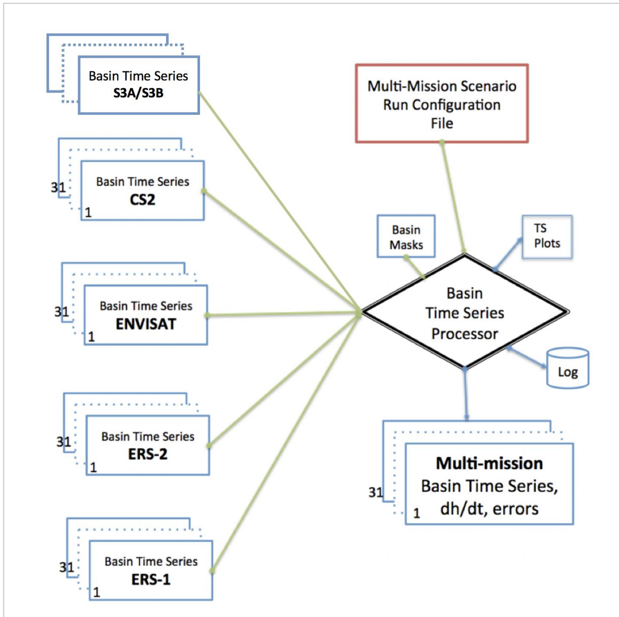
Figure 2.7: Multi-mission Basin Time Series Processor
