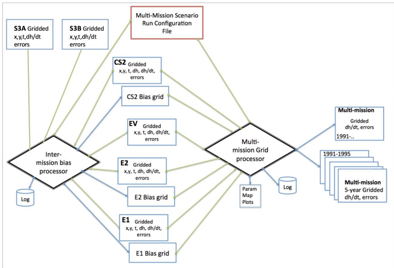
Figure 2.6: SEC Multi-mission dh/dt processor
