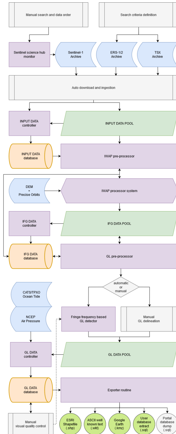
Figure 4.1: System overview flowchart: part one. Input data in light blue, processes in violet, database systems in orange, manual processes in grey, intermediate processing results in light green and products in lime green.
