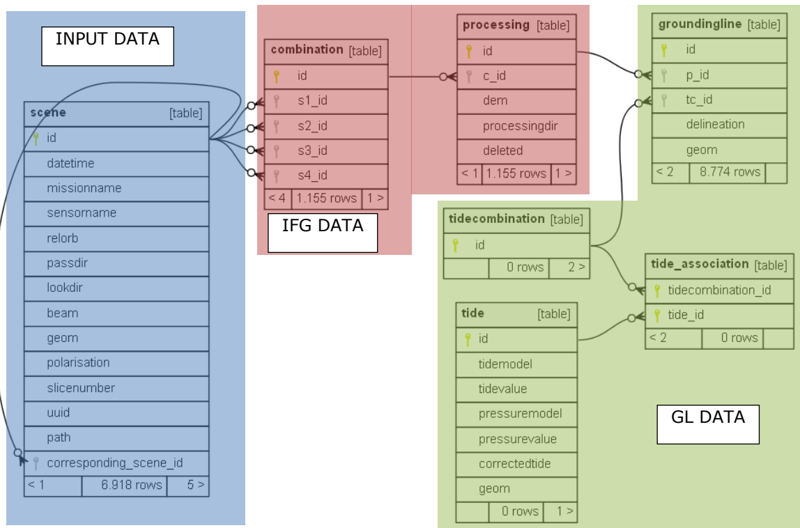
Figure 4.2: The PostGIS database structure containing information of the INPUT DATA, the IFG DATA and the GL DATA modules shown in Figure 4.1 .
