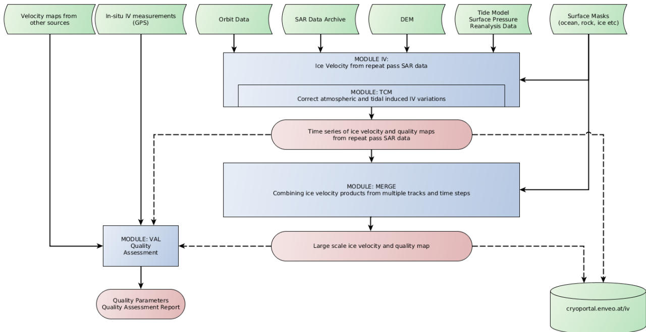
Figure 3.1: High-level flow chart of the ENVEO ESP 2.1 IV processing system. Green: input data, blue: processing modules, red: (intermediate) products.
