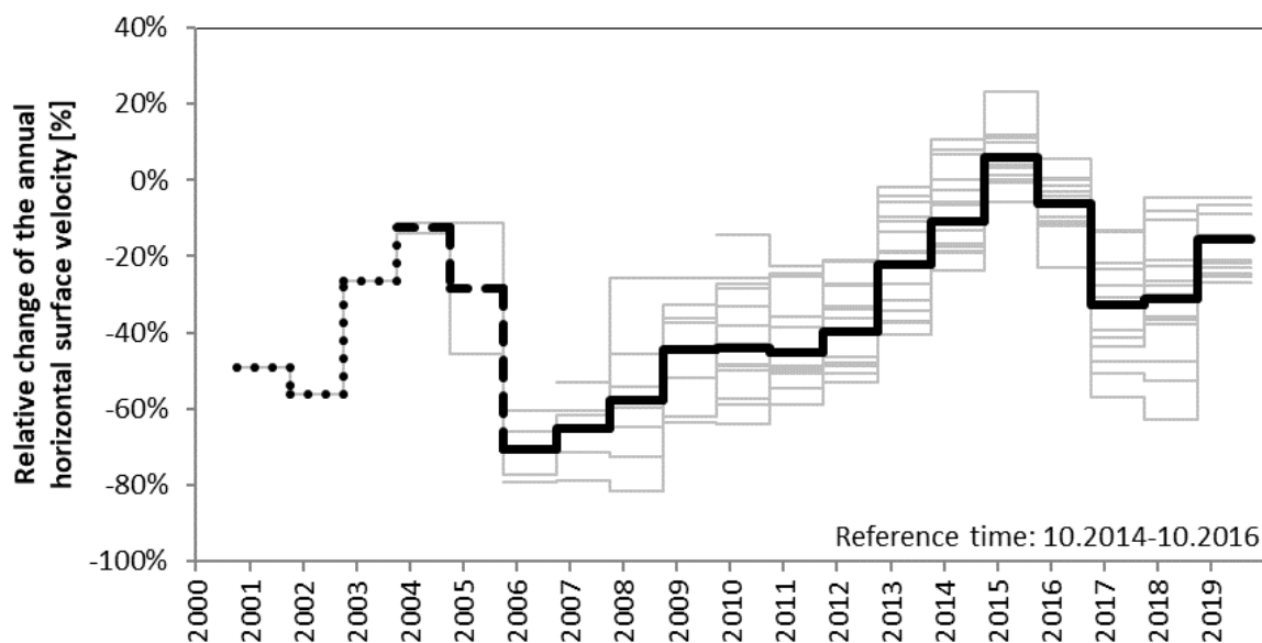
Figure 3: Relative change of the rock glacier surface velocity in the western Swiss Alps (data source: University of Fribourg, University of Lausanne, PERMOS): the regional index (black line) is the mean of selected individual rock glacier time series ( n = 1 to 14 according on years), which are derived from aggregated horizontal velocities based on annual GNSS multi-point surveys. Scale in % of change to a reference time. Measurement and calculation interval: 1 yr. The regional index is less significant when n is small, here drawn by small dots when n=1 and larger dots when n=2 .
